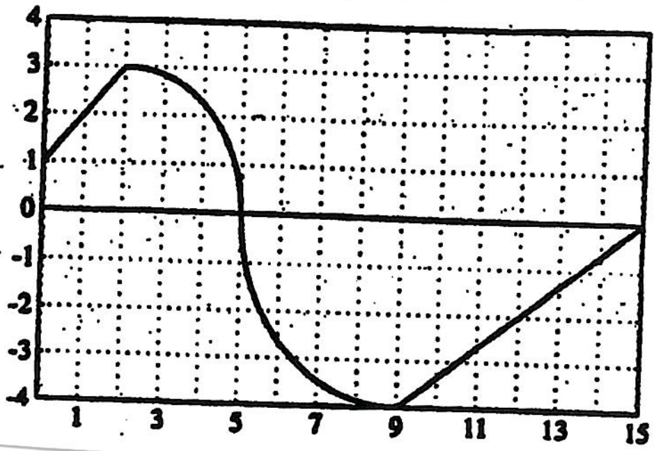
Graph of y = f(x)
